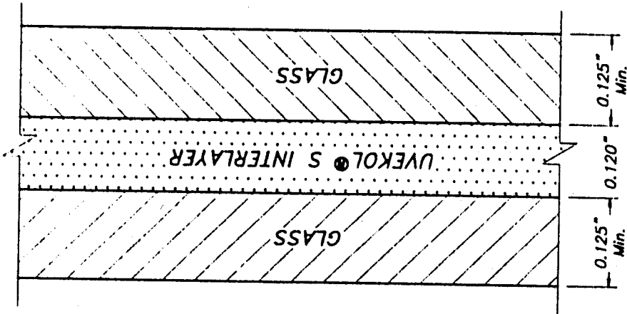
CROSS SECTION
